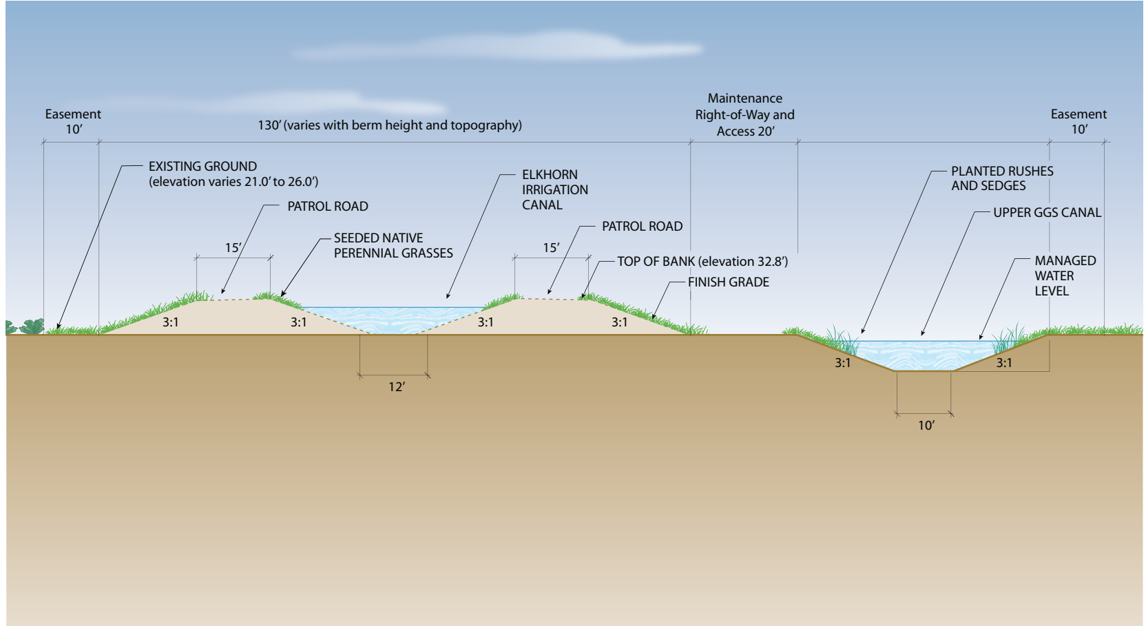
Typical Elkhorn Irrigation Canal and GGS/Drainage Canal
